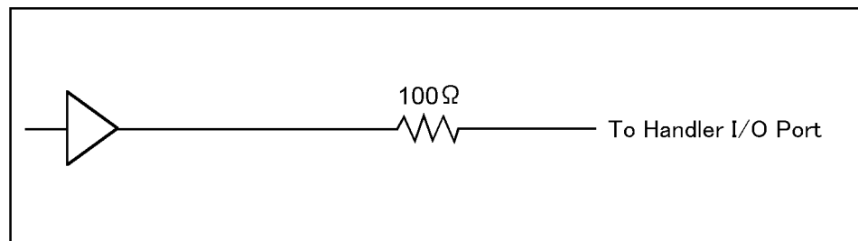
Figure 10-8 Circuit diagram of output signals
