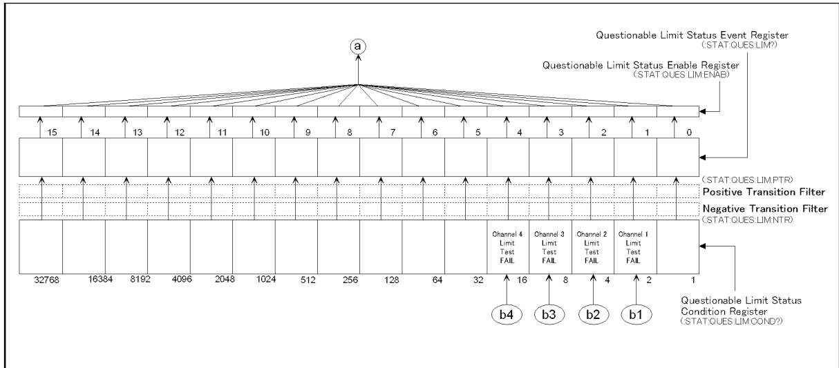
Figure B-4 Status Register Structure (2 of 7)
