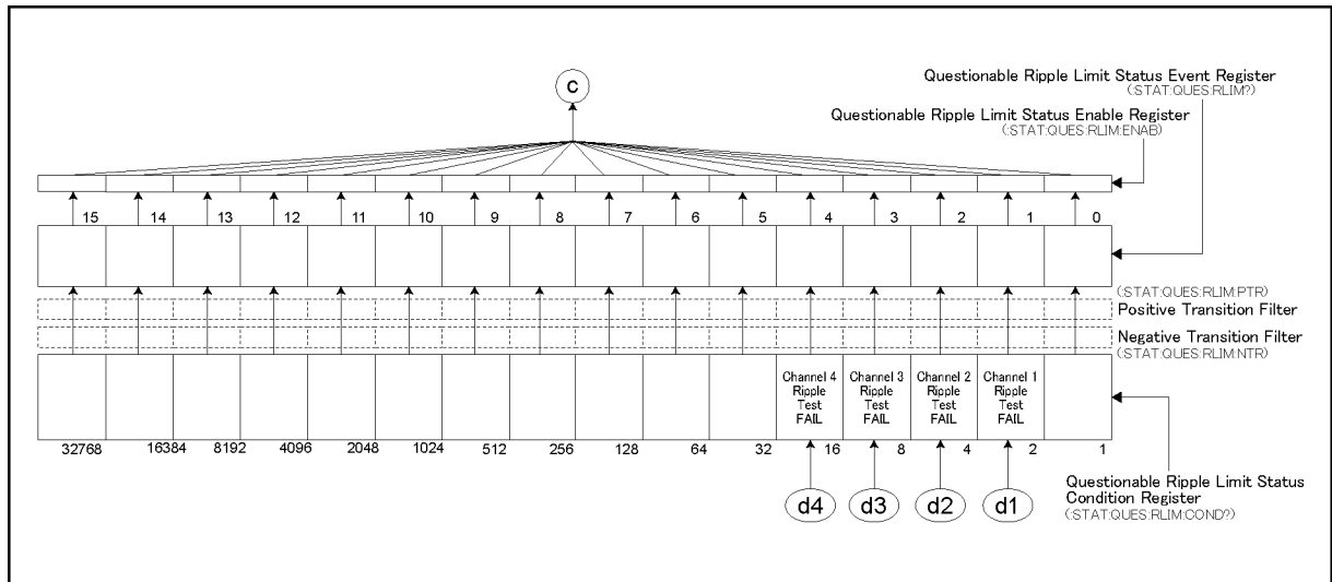
Figure B-5 Status Register Structure (3 of 7)
